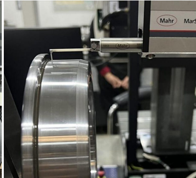
Roughness Tester
