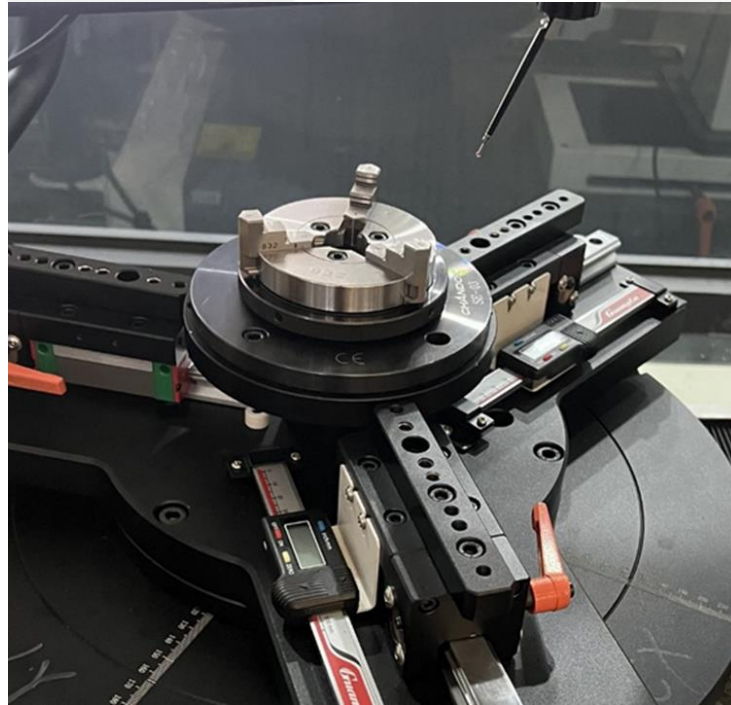
Roundness meter
