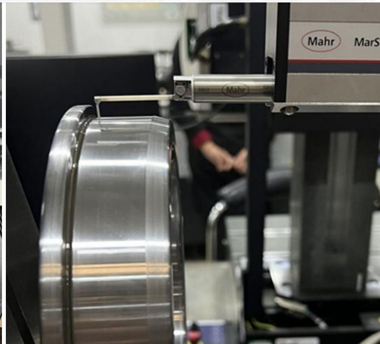
Roughness Tester
