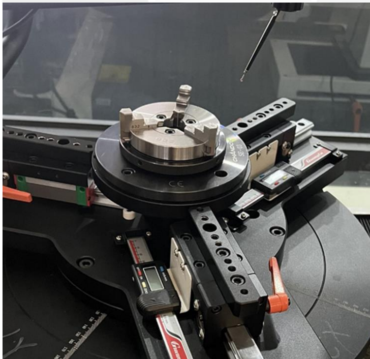
Roundness meter
