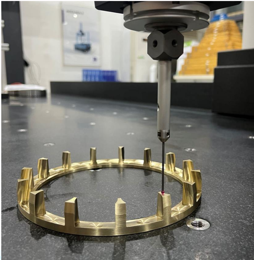
3D coordinate measuring instrument. For any complex shape, its geometric accuracy can be effectively inspected.
